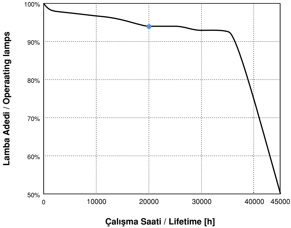
Lamba Çalışma Eğrisi / Typical lamp survival rate over lifetime
