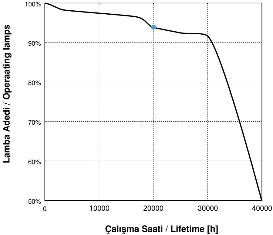
Lamba Çalışma Eğrisi / Typical lamp survival rate over lifetime
